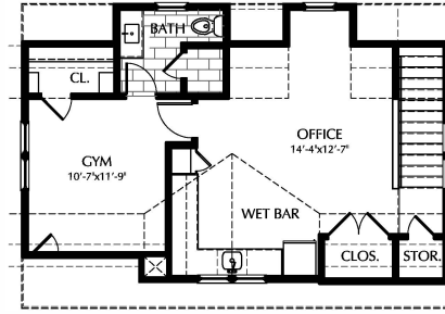
GARAGE SECOND FLOOR PLAN
