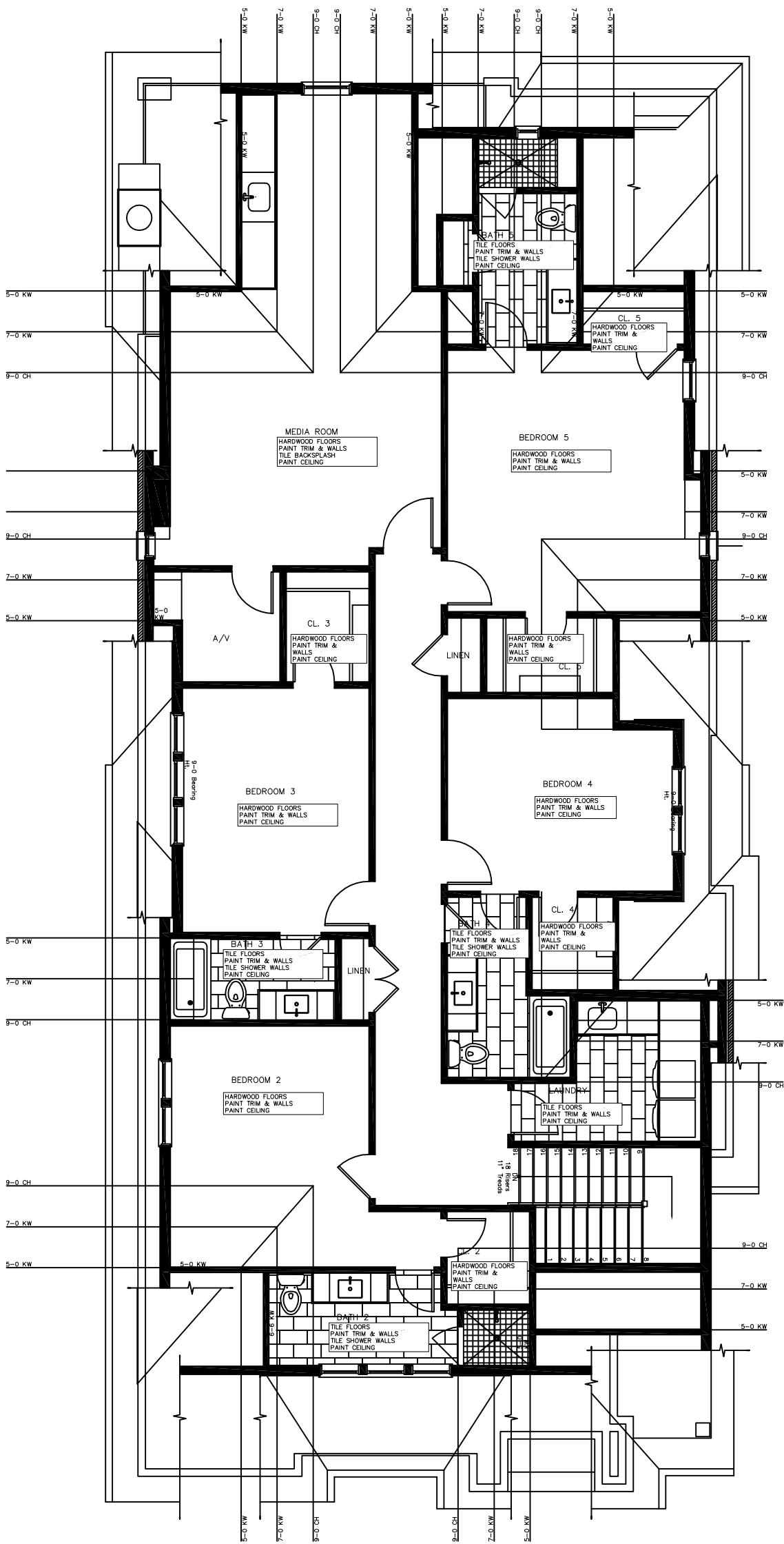
2ND FLOOR MATERIALS PLAN SCALE: \frac{1}{8}" = 1'
