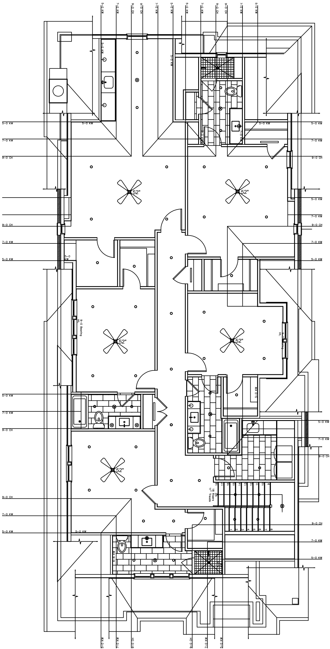
2ND FLOOR LIGHTING PLAN SCALE: \frac{1}{8}" = 1'
