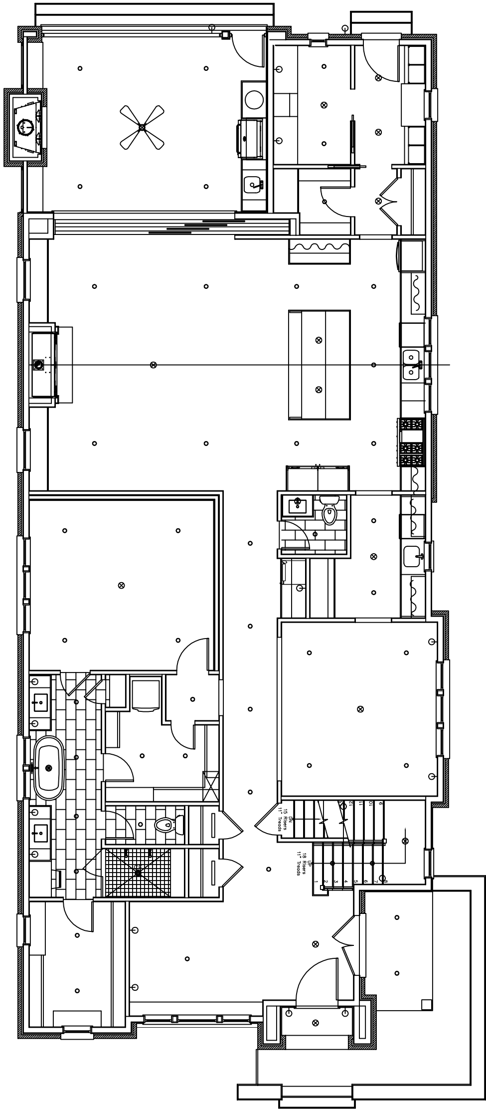
1ST FLOOR LIGHTING PLAN SCALE: \frac{1}{8}" = 1'
